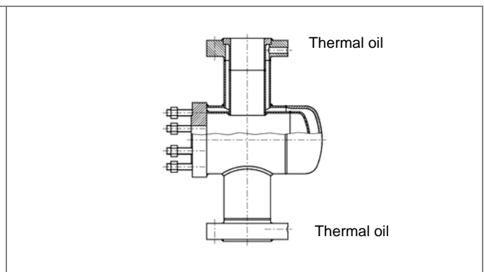
fig. 2 Double-walled float chamber for thermal oil heating
